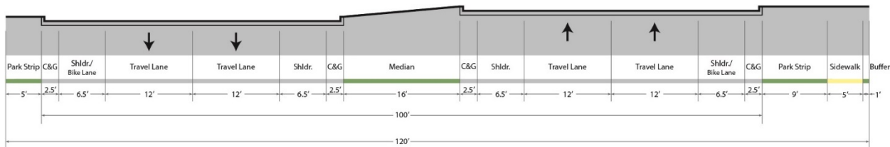
Figure 4-14. Cross Section, Highland Drive Arterial B
